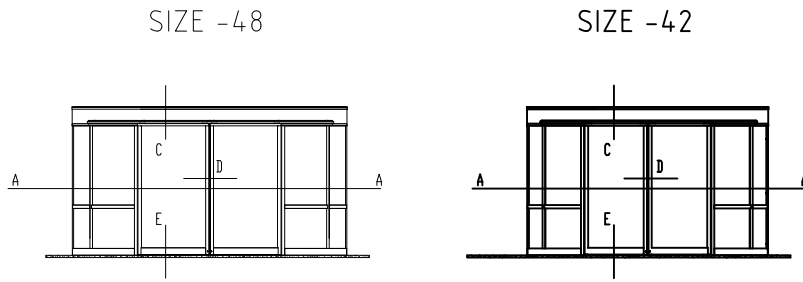
FRONT VIEW (CLOSED DOOR)
